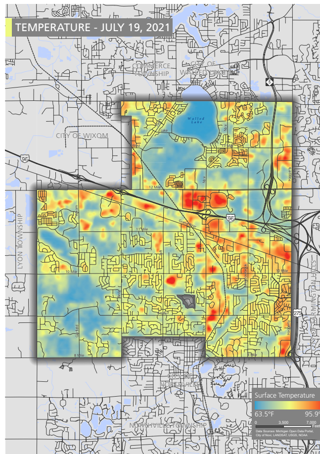
Map 3: Temperature - July 19, 2021
