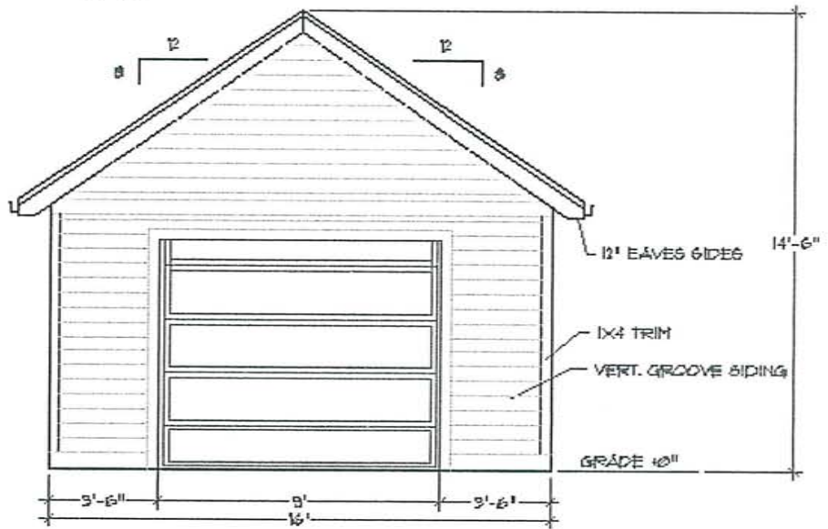
FRONT ELEVATION W-1-0"
